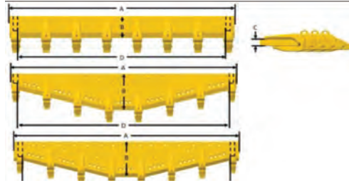
Base Edge Assembly Dimensional Reference
